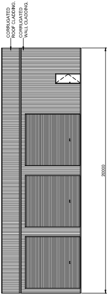
1 SIDEWALL EXTERIOR ELEVATION SCALE: 1 = 200
